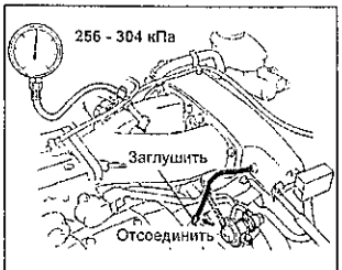
2JZ-GE.
