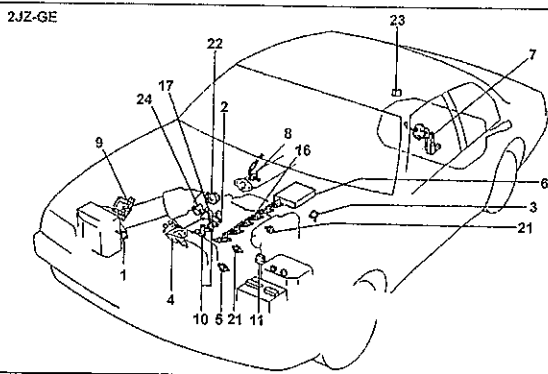
2JZ-GE
