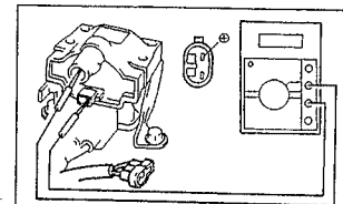
1JZ-GE, 2JZ-GE.
