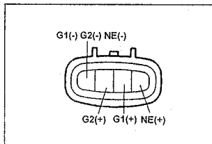
1JZ-GE, 2JZ-GE.
